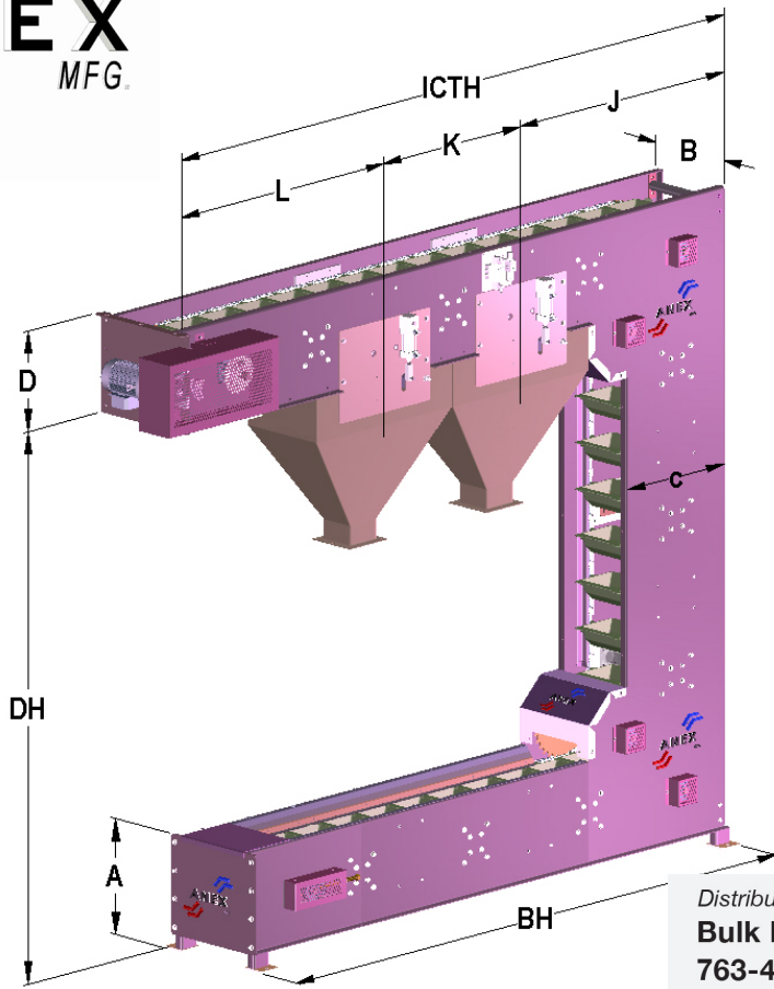
SOLID WALL BUCKET ELEVATOR-IDS-“C”
