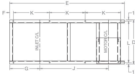
FOUNDATION PLAN
